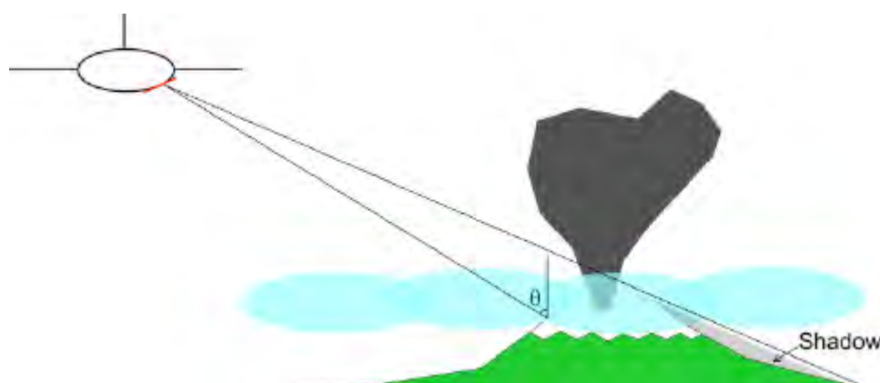
Figure 4.26. The imaging arrangement of the airborne Synthetic Aperture Radar (SAR) which enabled data acquisition through clouds and ash plumes. \theta designates the incidence angle for a target in the near range of the SAR.
