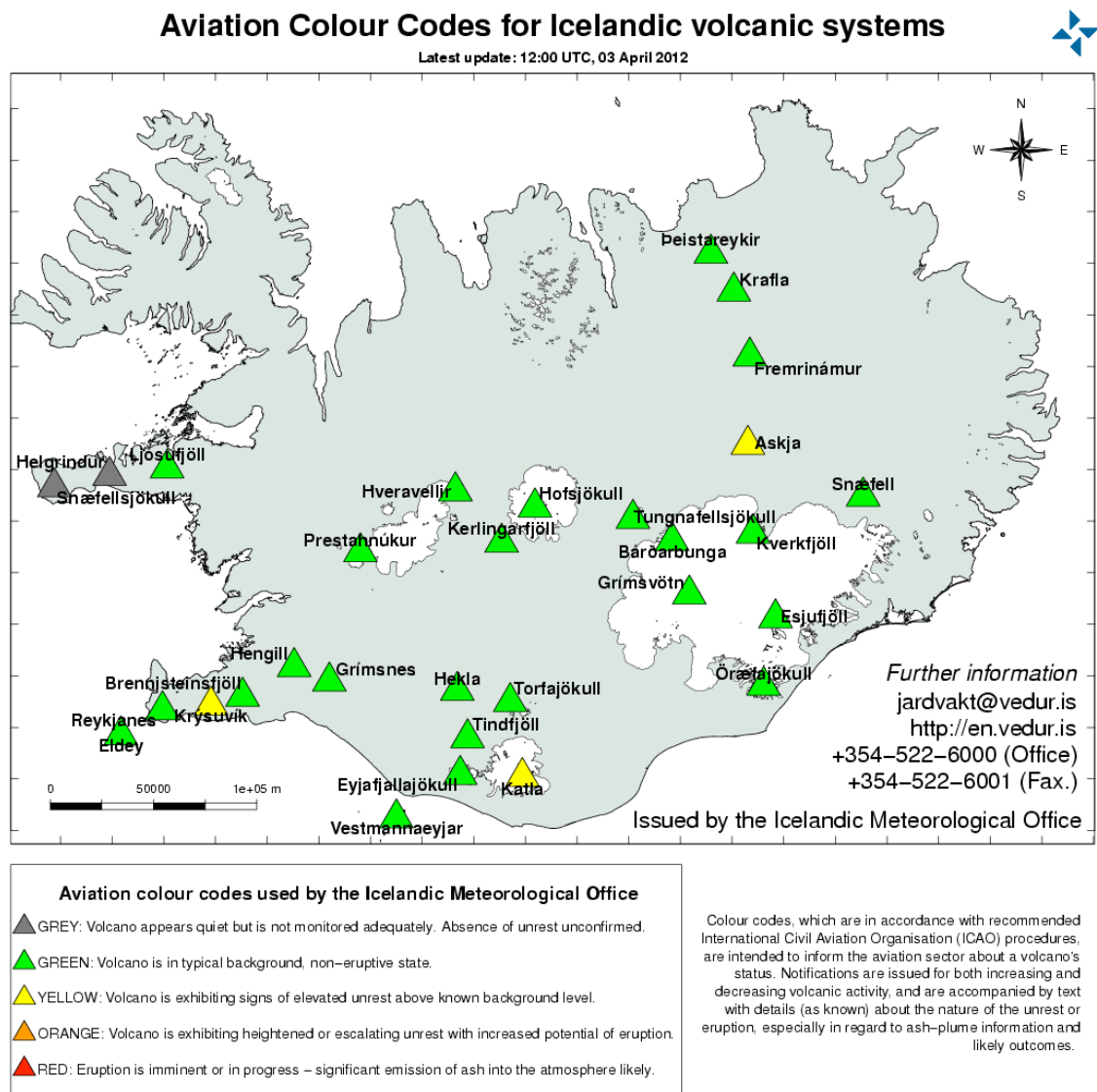
Figure 5.9. A preliminary map of Aviation Color Codes for volcanic systems in Iceland.
